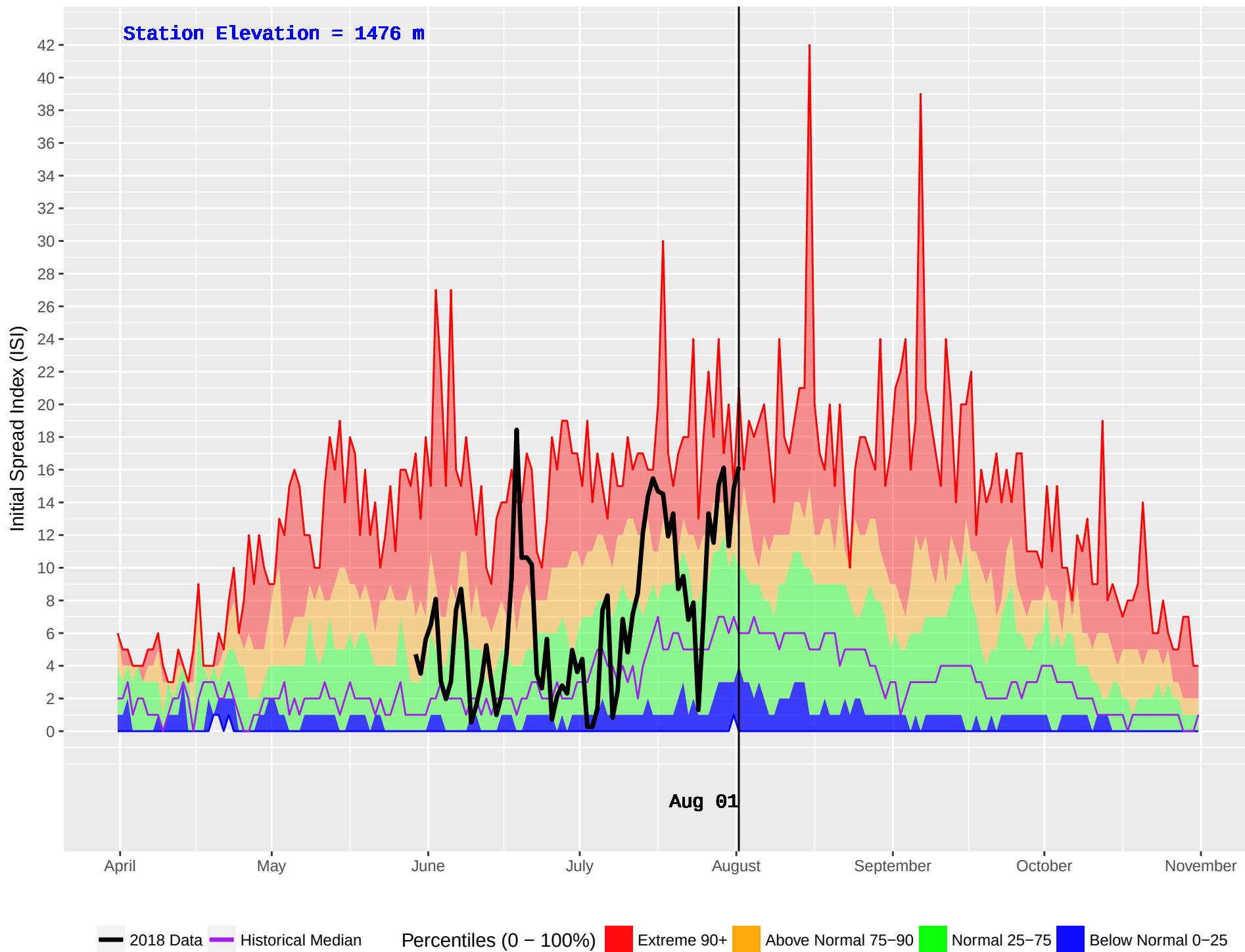
BRENDA MINES (283) : Historical (1977–2016) and Current (2018) Daily Initial Spread Index (ISI)
