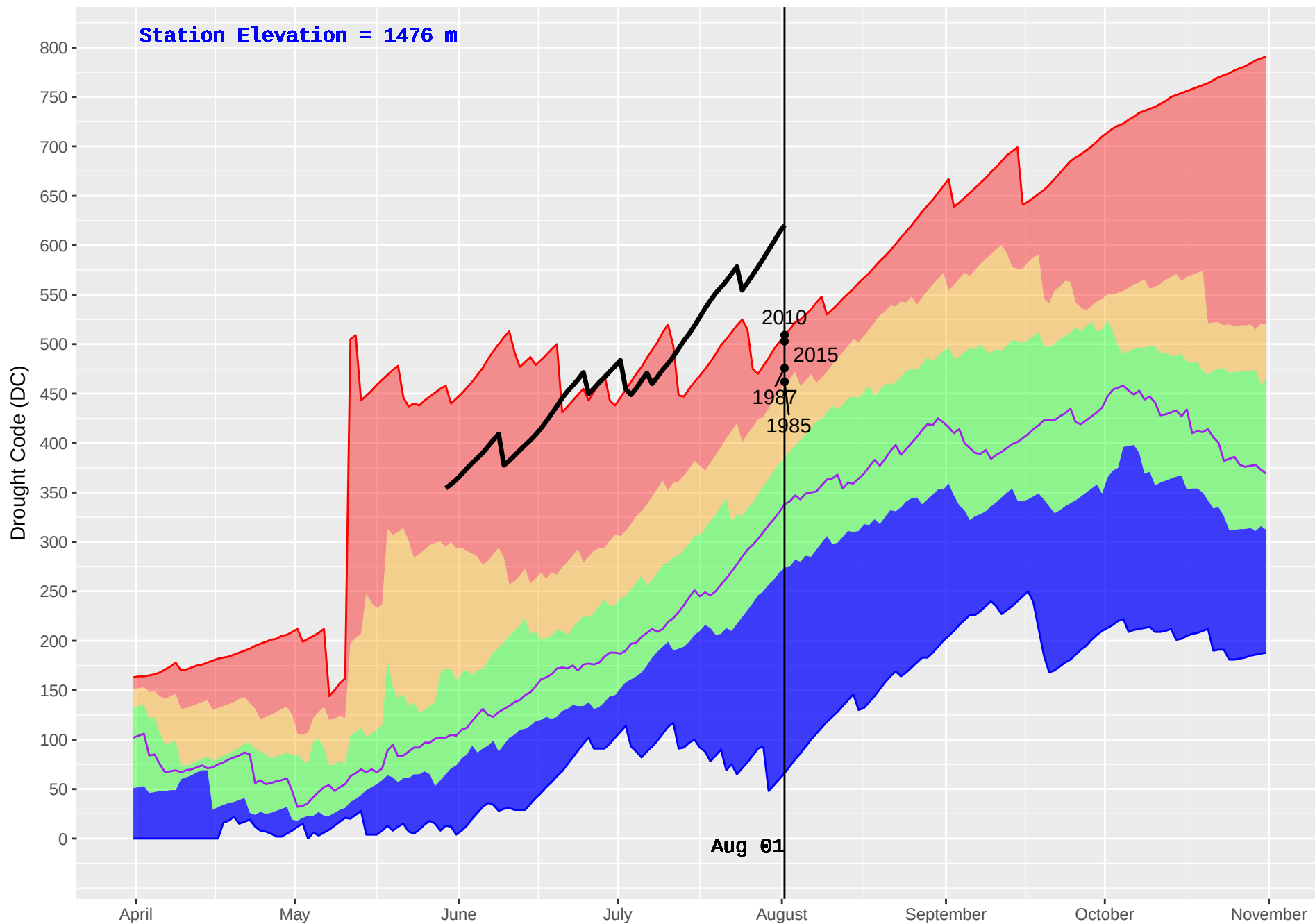
BRENDA MINES (283) : Historical (1977–2016) and Current (2018) Daily Drought Code (DC)
